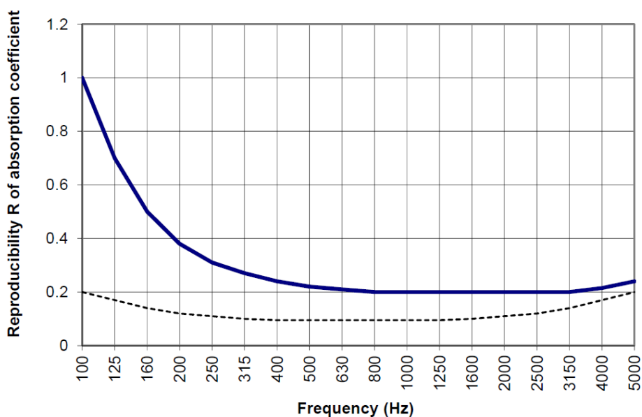
Figure 3.2: Assessment of absorption coefficient reproducibility R from ISO 354-2003(E) – for absorbers with high absorption coefficients ( \alpha_w = 1.00 ) in all bands (continuous line) and for absorbers with low absorption coefficients ( \alpha_w = 0.05 ) in all bands (dashed line).
